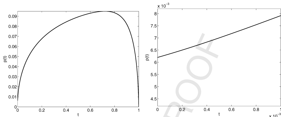
Fig. 6. Numerical solution of (4.3)–(4.5) for a_0 = 1 , b_0 = 2 , \gamma = 1.4 . Left graph: p(t) , t \in [0, 1] ; right graph: p(t) , t \in [0, 10^{-3}] .
